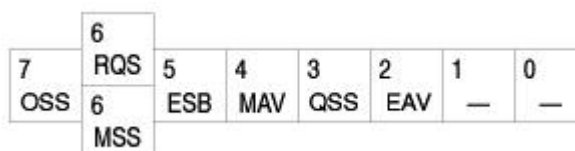
Figure 9: The Status Byte Register (SBR)
